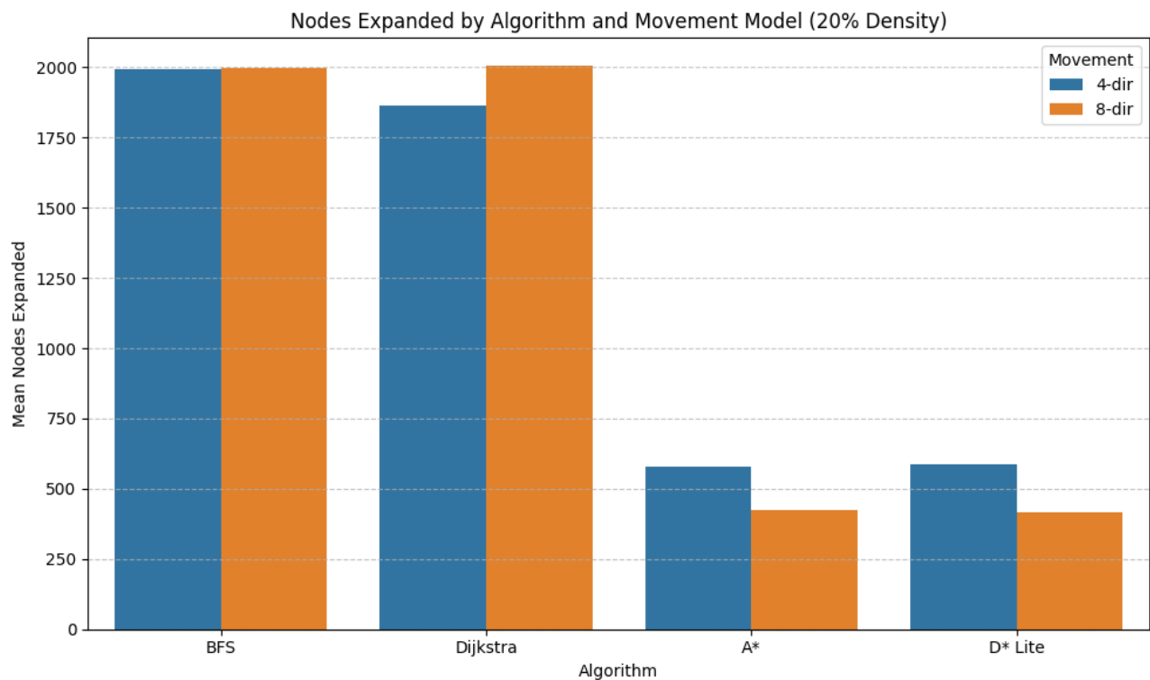
Fig 4.3.2: Effect of movement model on the node expansion
